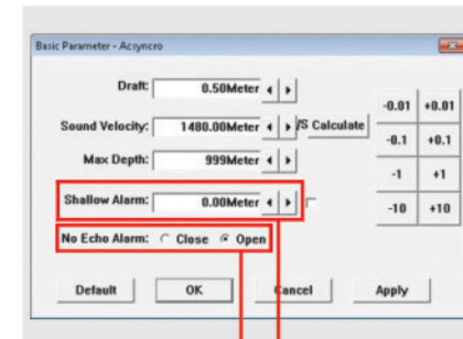
"No Echo" Alarm Shallow-water Alarm
